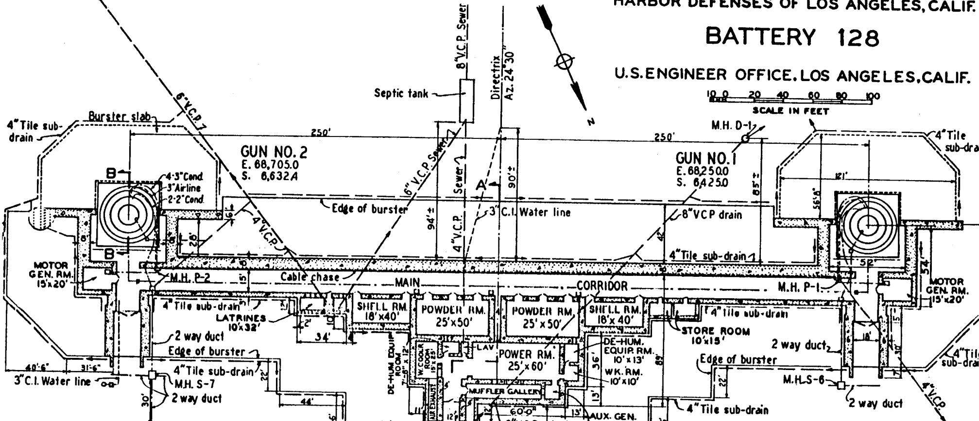
PLAN
