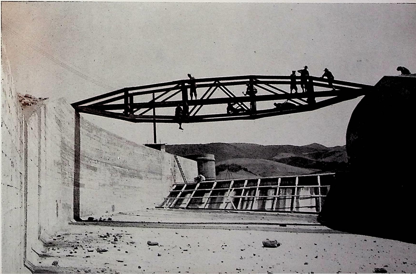
COMPLETED FOOTBRIDGE (SHOWN ON FACING PAGE) WHICH GIVES THE TROOPS PASSAGE ACROSS RESERVOIR
