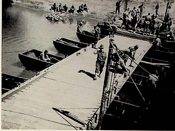
A pontoon bridge crossing is erected.
