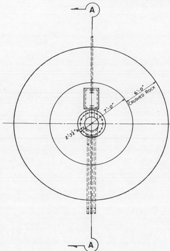
PLAN OF GUN BLOCK
